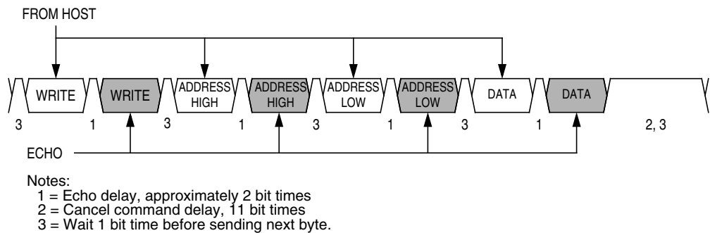
Figure 7-5. Write Transaction
