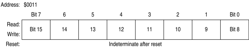
Figure 8-12. TIM Channel 0 Register High (TCH0H)
