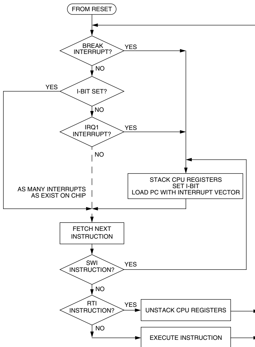
Figure 6-10. Interrupt Processing
