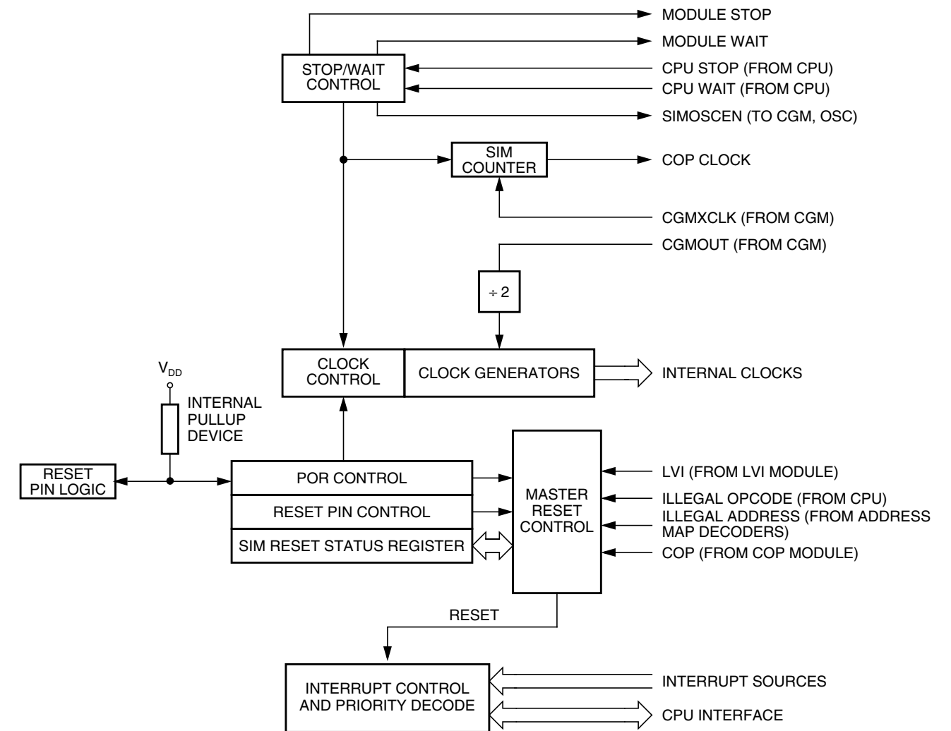
Figure 6-1. SIM Block Diagram
