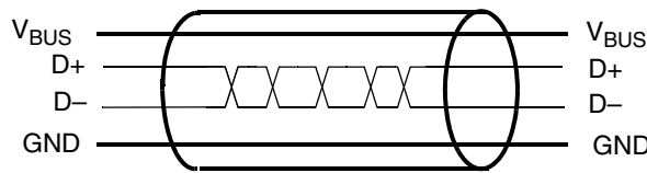
Figure 2. USB Lines — Data (D+, D-) and Power Supply (VBUS, GND)
