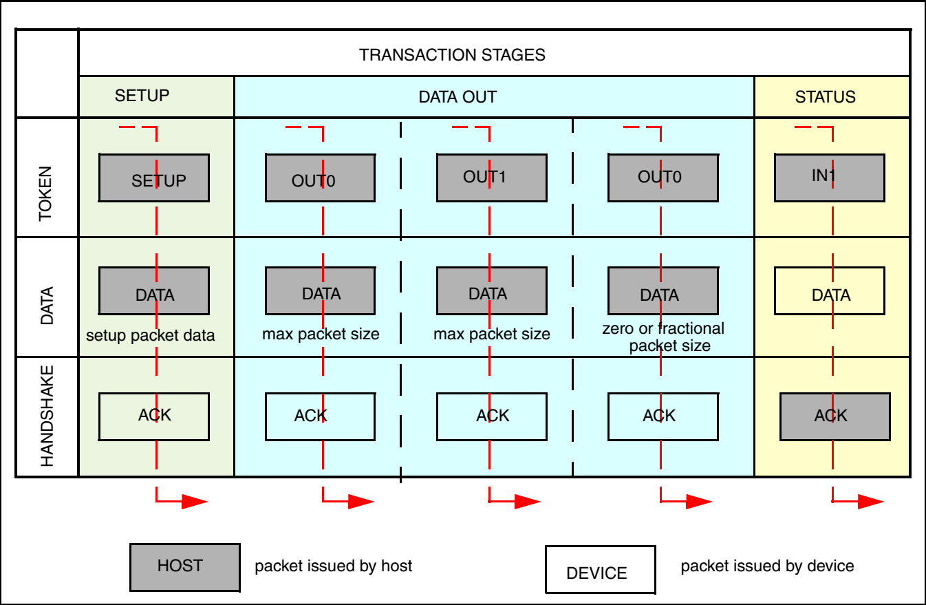
Figure 10. Control OUT Transaction — All Packets
