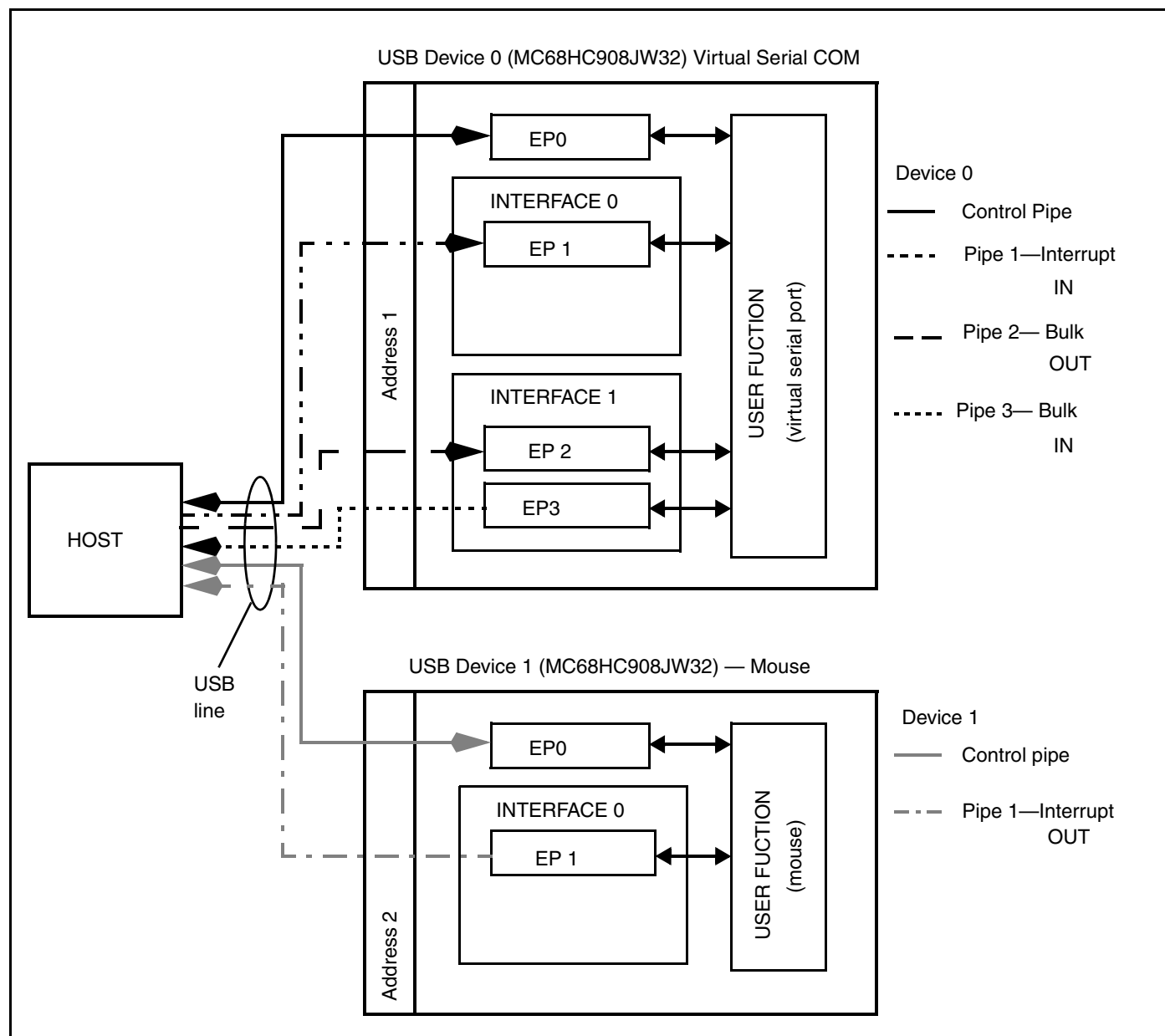
Figure 5. USB Logical Structure — Endpoints and Pipes
