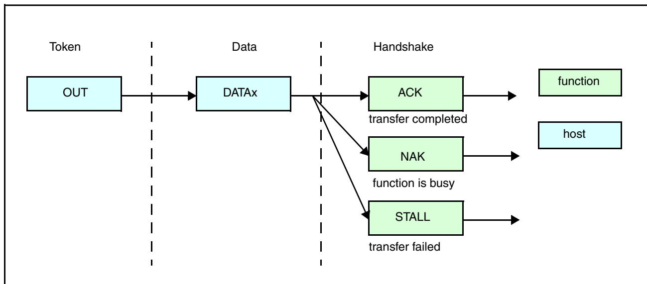
Figure 18. Bulk/Interrupt OUT Transfer — All Packets
