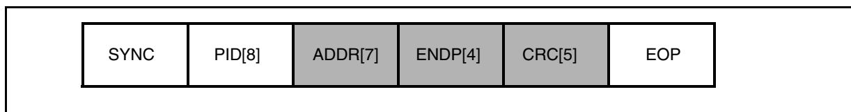
Figure 6. Token Packet Fields
